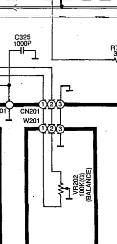
D BALANCE VR CIRCUIT (P.C. Board: on page 10)
