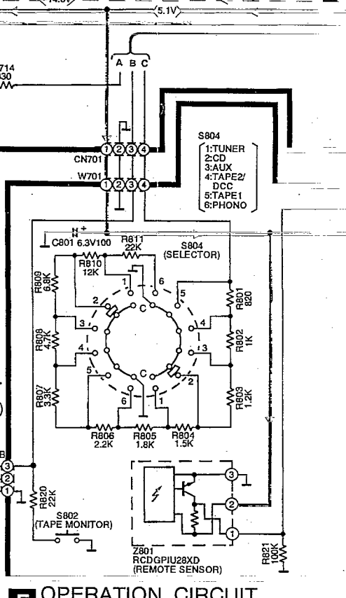
F OPERATION CIRCUIT (P.C. Board: on page 10)
