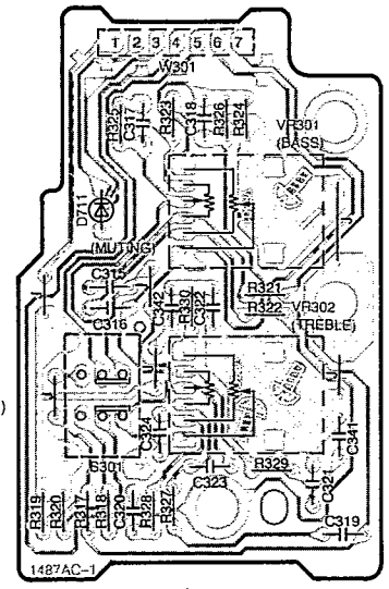
B TONE SWITCH P.C.B. (REP2156A-2S)
