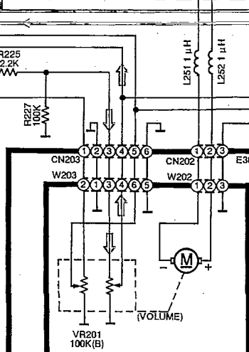
C VOLUME CIRCUIT (P.C. Board: on page 10)
