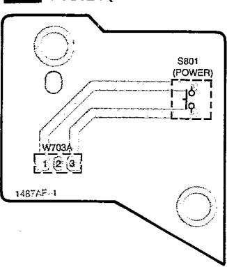
E POWER SWITCH P.C.B. (REP2156A-2S)
